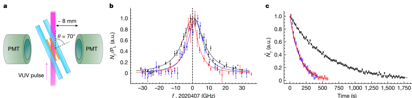
Fig. 2 | Nuclear spectroscopy of the ^{229}\text{Th} clock transition in the ^{229}\text{ThF}_4 film.
