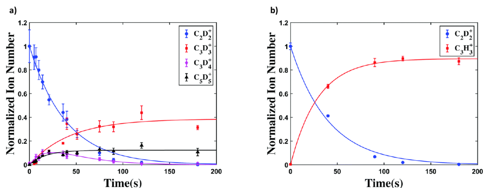
Figure 6. Normalized relative populations of m/z as measured by mass spectrometry, plotted with respect to the time exposed to the neutral reactant. (a) Reaction C_2D_2^+ + DC_3D_3 produces multiple primary products: C_3D_3^+ , C_3D_4^+ , and C_3D_5^+ . Note that C_3D_4^+ further reacts with DC_3D_3 to form the second-order products C_6H_5^+ and C_6H_7^+ , which are not shown in this figure. (b) Reaction C_2D_2^+ + H_2C_3H_3 . Most of the products are C_3H_3^+ . While a very small amount of C_3H_4^+ is also produced, it undergoes a secondary reaction fairly quickly and does not accumulate in significant numbers. Adapted with permission from Schmid et al. 51 Copyright 2020 PCCP Owner Societies.
