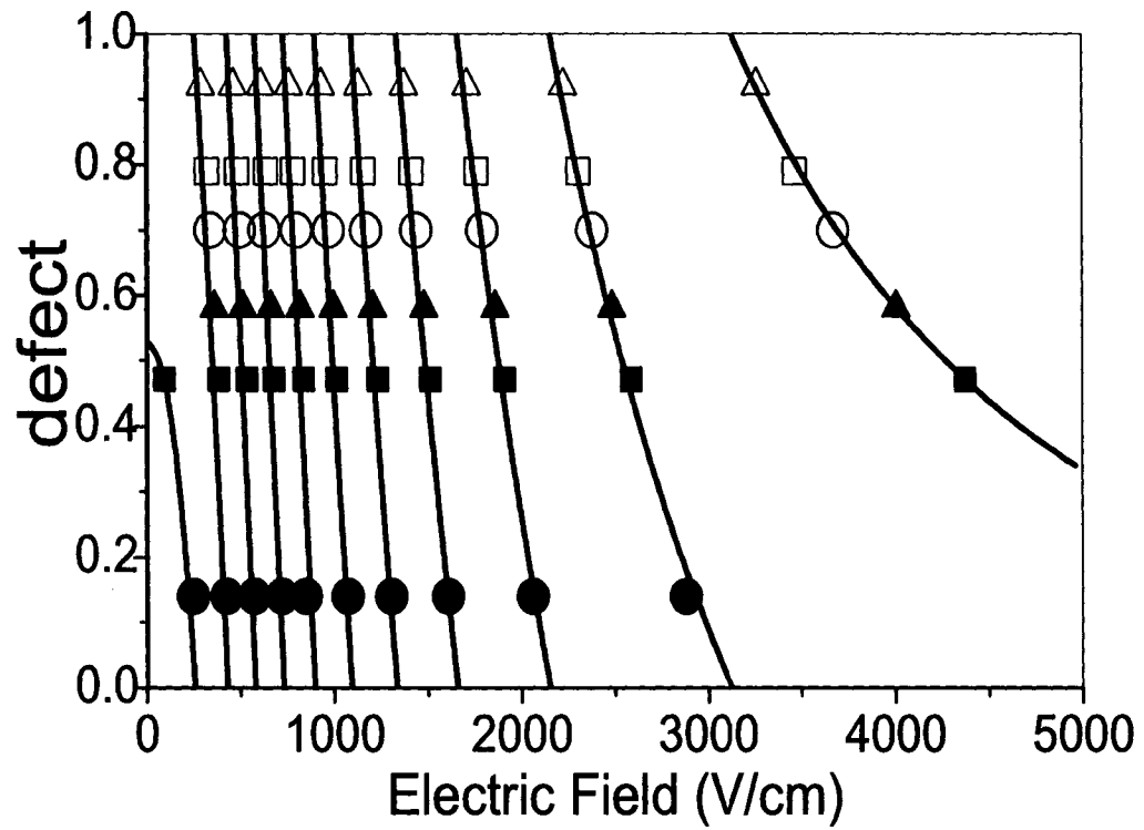
Figure 5.6: The vertical curves represent electric field values where the AWP predicts potential resonances for a given defect, \mathcal{E}_{WKB}(\delta_{defect}) . The points represent resonant field values, \mathcal{E}^{(b)} , in the full calculations with different initial boundary conditions. The values of b are given by \cotan(\pi\beta) . The values of \beta for the different full numerical calculations are 0 (filled circle), 0.11 (filled square), 0.22 (filled triangle), 0.56 (hollow circle), 0.78 (hollow square), and 0.89 (hollow triangle). Each set of values \mathcal{E}^{(b)} is plotted at a height corresponding to its best-fit value of \delta_{defect} .
