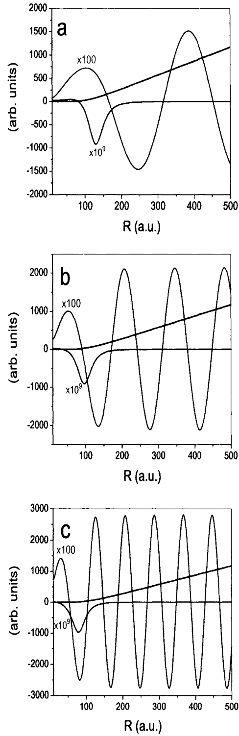
Figure 4.7: Illustrations of the origin of the zero in the partial rates. Each panel shows curves \psi_l , \frac{d}{dR}\psi_\varphi \times 100 and P_{\nu\varphi} \times 10^9 . The plots are for different final energies, and the inelastic rate from the Born approximation are (a) E_f = -6mK and K_{\nu\varphi}^{inel} = 5 \times 10^{-11}(cm^3/s) , (b) E_f = -22mK , K_{\nu\varphi}^{inel} = 5 \times 10^{-14}(cm^3/s) , and (c) E_f = -62mK , K_{\nu\varphi}^{inel} = 6 \times 10^{-13}(cm^3/s) , see text for details.
