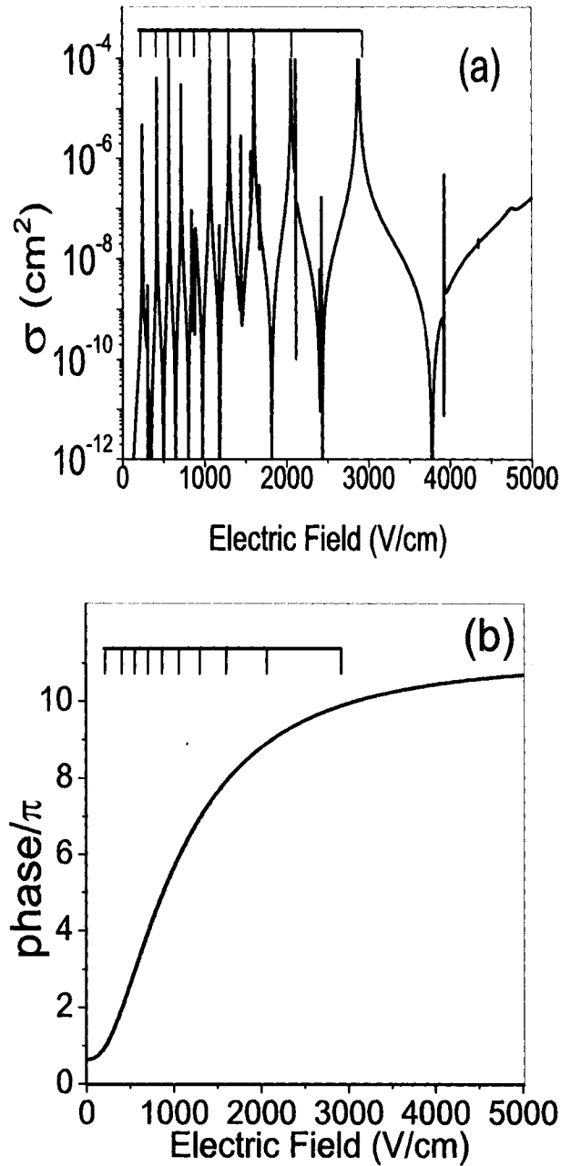
Figure 5.4: (a) Cross section for RbCs in strong-field seeking states, including the 10 potential resonances that the AWP predicts (solid bracket). The AWP phases are shown in (b). The black bracket corresponds to the AWP predicted resonances for the lowest adiabatic curve after a defect, \delta_{\text{defect}} = 0.14 , has been added according to Eq. (5.4). The gray triangles are the AWP predicted resonances without the defect.
