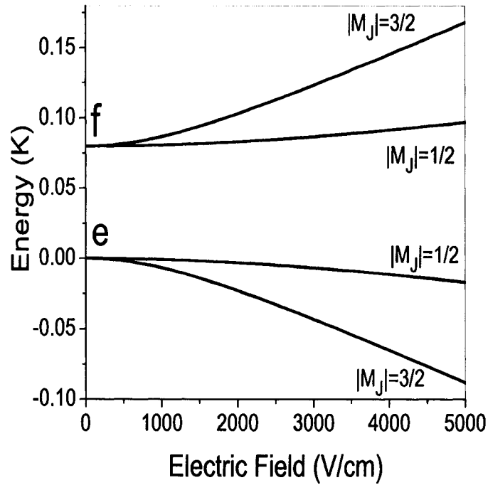
Figure 2.2: The Stark effect for OH excluding hyperfine structure, with its ^2\Pi_{3/2} ground state. We have set the \Lambda -doublet energy equal to 0.08 (K) and electric dipole of \mu = 1.668 (D) [87]. One key feature of this plot is that at low field, the energies vary quadratically and then vary linearly at high field once the Stark energy is larger than the splitting. This transition happens at roughly 1000 (V/cm) for OH [87].
