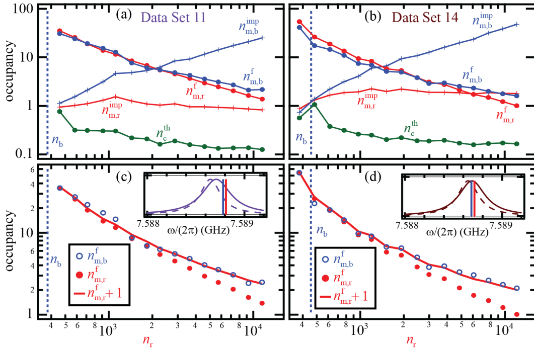
Figure 9.3: Measured sideband asymmetry as a function of red-drive photon number for data set 11 (a,c) and data set 14 (b,d). The cavity response and sideband frequencies for each data set are shown as insets. (a,b) Inferred final mechanical occupancies, imprecision, and thermal cavity occupancy as a function of number of red-drive photon number. (c,d) Comparison of upper red and lower blue final sideband occupancies. The lower blue occupancy is scales such that the red and blue occupancies are equal for the lowest power. The red line is the red data plus one.
