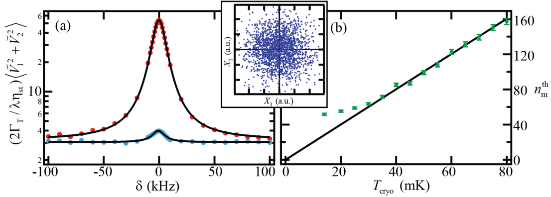
Figure 11.3: Calibration of phonon units and apparent mechanical motion. (a) The apparent motion (imprecision) can be calibrated by calculating the inferred mechanical occupancy with the basis functions detuned by |\delta| \gg \Gamma_T from the frequency of optimal inference. (b) The conversion factor between measured voltage and inferred mechanical occupancy can be calibrated by measuring the mechanical oscillator in equilibrium with its bath as a function of cryostat temperature. (inset) Each point in the temperature sweep consists of 2000 inferences of the mechanical state.
