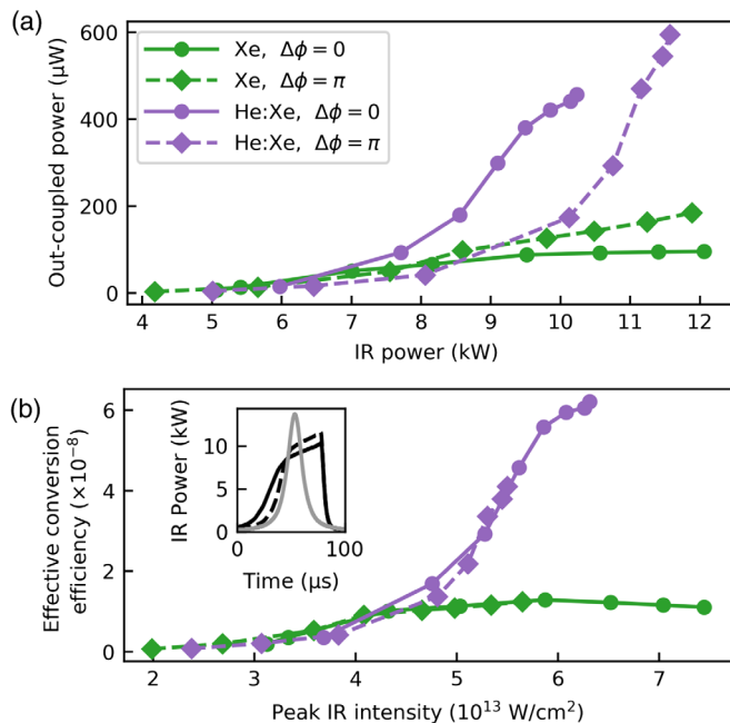
FIG. 5. (a) Out-coupled 11th harmonic power (back-calculated to the point right after the out-coupling mirror pair, see Supplemental Material [52]) as a function of intracavity (single beam) fundamental drive power, shown for different generation media and relative phases. Data is taken when the cavity is swept across the resonance. As shown in Ref. [12], similar harmonic power is expected when the cavity is locked with a similar intracavity power level. (b) Effective conversion efficiency (defined in the text) as a function of peak drive intensity. Inset shows intracavity IR power when the cavity is swept across a resonance, with \Delta\phi = 0 (continuous black) and \Delta\phi = \pi (dashed black) configurations using a He:Xe mixture gas target, displaying clear deviations from the Lorentzian line shape obtained without a gas target (gray), indicating significant plasma density. Green traces are recorded with pure Xe with 260 kPa backing pressure at room temperature. Purple traces are recorded with 9:1 He:Xe mixture with 4100 kPa backing pressure heated to \sim 560^\circ\text{C} .
