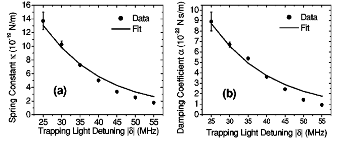
FIG. 3. Dependence of (a) \kappa and (b) \alpha on the trapping light detuning for a trapping beam intensity of 25 mW/cm ^2 and \partial B/\partial x = 26 G/cm. Fits are shown as solid lines.
