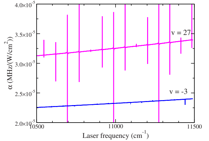
FIG. 7. (Color online) Real part of the dynamic polarizability of the J=0 vibrational levels of the \text{Sr}_2 X^1\Sigma^+ state as a function of laser frequency in the range of 10\,500\text{--}11\,500\text{ cm}^{-1} . For clarity, only two selected vibrational levels of the X state are shown, v = -3 and v = 27 . The polarizabilities are evaluated at 0.1\text{-cm}^{-1} intervals. The polarizabilities of J=0 rotational levels are independent of the laser polarization.
