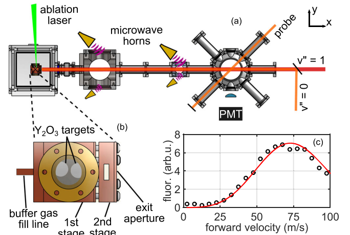
FIG. 2 (color online). (a) Depiction of the beam apparatus. The YO molecular beam interacts with a counterpropagating slowing laser beam along x . A 45^\circ probe beam is used for Doppler sensitive detection. A photomultiplier tube (PMT) is used to collect fluorescence induced by either the slowing or probe beam. (b) Two-stage buffer-gas cell. (c) Velocity distribution measured at the detection region. The solid line is a fit to a Gaussian (with center longitudinal velocity of the beam at 49 m/s and a temperature of 8 K) multiplied by the square of the forward velocity to account for the transverse velocity spread.
