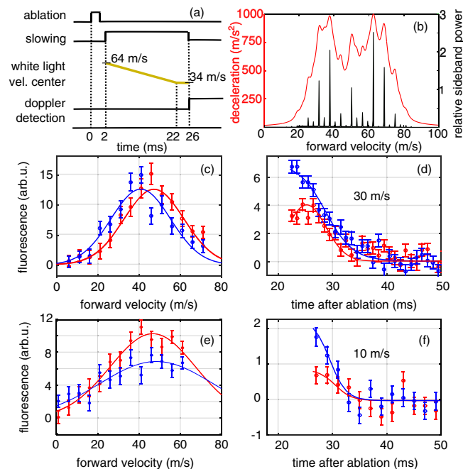
FIG. 4 (color online). (a) Timing sequence used to slow molecules to below 10 m/s. (b) Example of spectrally broadened slowing light with center velocity of 50 m/s. Black lines show the sidebands generated from an electro-optic modulator and rapid polarization switching. The red curve shows molecular deceleration with an optical saturation parameter of 3. (c)–(f) Comparisons between no slowing in red and with slowing in blue. Solid lines are guides to the eye. (c) Doppler spectra for a 10 ms long slowing sequence. (d) Time of flight for 30 m/s molecules. (e) Doppler spectra for a 24 ms long slowing sequence as depicted in (a). (f) Time of flight for 10 m/s molecules.
