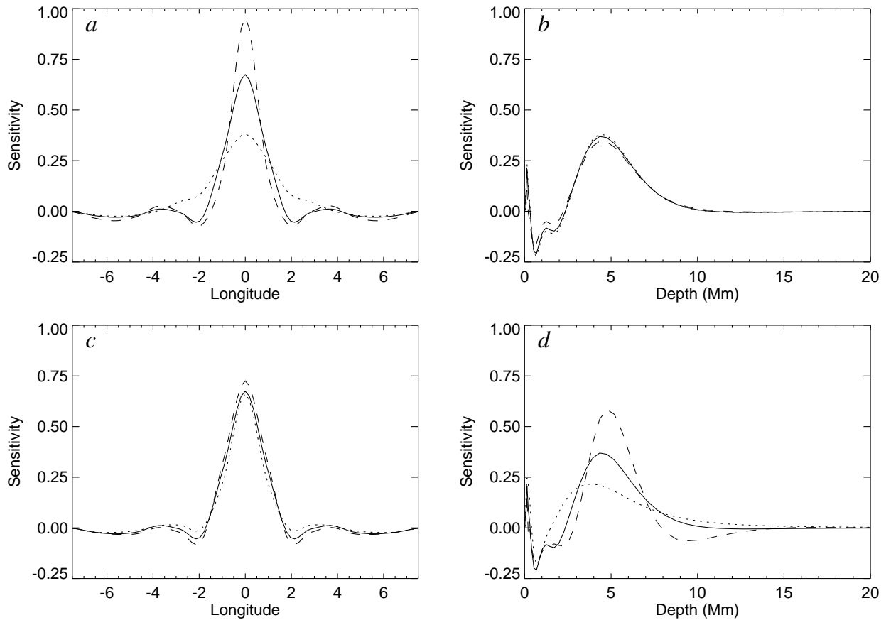
Figure 7.9: Sensitivity of the averaging kernels to variations in the regularization for an averaging kernel targeted at the 5 Mm depth. (a,b) Variation of the (a) horizontal and (b) vertical structure of the averaging kernel with changing horizontal regularization. \lambda_v has been taken to be 0.1. \lambda_h of 0.1, 1.0, and 10.0 are indicated by dashed, solid and dotted lines, respectively. (c,d) Variation of the (c) horizontal and (d) vertical structure of the averaging kernel with changing vertical regularization and \lambda_h of 1.0. \lambda_h of 0.01, 0.1, and 1.0 are indicated by dashed, solid and dotted lines, respectively. Variations in \lambda_v change the vertical structure of the averaging kernels while leaving the horizontal structure relatively unchanged. Similarly, \lambda_h primarily affects the horizontal structure of the averaging kernels.
