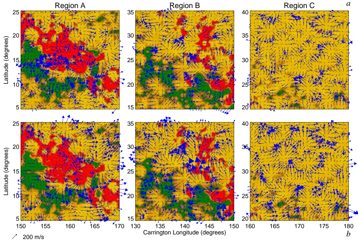
Figure 8.2: Closeups of the regions of interest indicated by white lettering in Figure 8.1 for the ( a , upper row) ARRI results and the ( b , lower row) 2^\circ f -mode fits. Detailed examination of the flow structures in quiet sun (Region C) reveals good agreement between the two datasets. In more active regions (such as A,B), data dropouts are present in the 2^\circ f -mode data set (visible as small blue dots). The 3-D inversion uses 4^\circ and 16^\circ degree data to reconstruct the solution where there is an absence of 2^\circ data.
