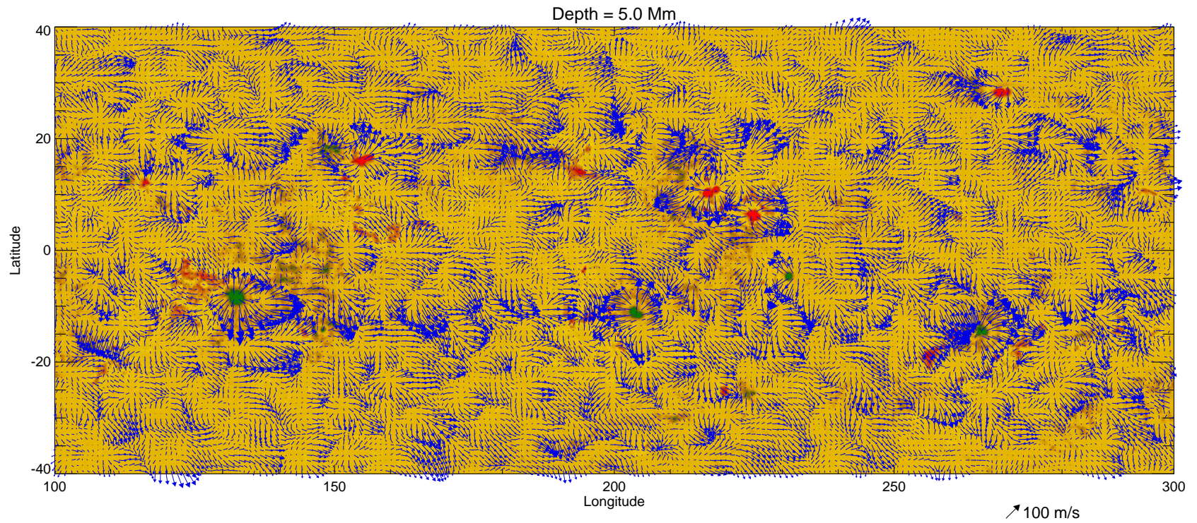
Figure 8.7: Synoptic map of Carrington rotation 1985 spanning the period 11 Jan 2002 through 25 Jan 2002 at a depth of 5 Mm as measured using ARRDI. Daily flowmaps obtained using full-disk stitched inversions were averaged in time over the this period. Each flow vector represents a seven-day average of the flow at that latitude and Carrington longitude. Sunspots, visible as dark green and red spots on the map, are home to strong 100 \text{ m s}^{-1} outflows. The torsional oscillations are visible at this depth as strong longitudinal flows in the activity belts.
