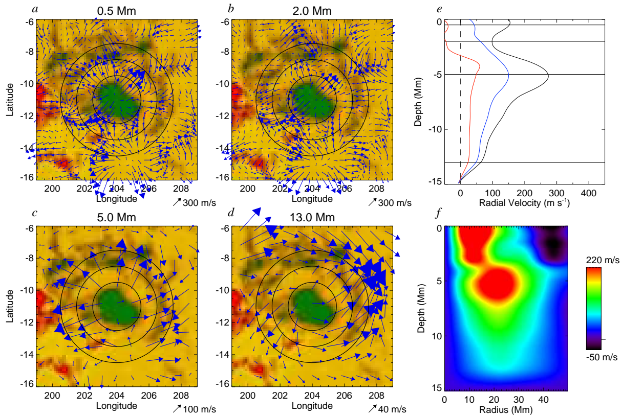
Figure 8.8: The depth variation of a sunspot outflow. (a-d) Horizontal flow beneath NOAA AR 9783 on 17 Jan 2002 at four representative depths as determined with ARREDI. Concentric circles indicate radii of 18, 30, and 42 Mm relative to the sunspot center. (e) Depth variation of the radial outflow (shown positive), averaged in angle around the sunspot center, is indicated at radii of 18 Mm (black), 30 Mm (blue), and 42 Mm (red). Solid horizontal lines correspond to the depths indicated in a-d. (f) 2-D view of the sunspot outflow with radius and depth. 150 \text{ m s}^{-1} outflows are visible at the surface and diminish in strength around 3 Mm. Outflows increase to 350 \text{ m s}^{-1} around 5 Mm before decaying steadily with depth. The sunspot outflows decay steadily with distance at all depths. A near-surface inflow is visible at the perimeter of the surface moat flow. Flow fields have been interpolated by a factor of two in all cases for ease of viewing.
