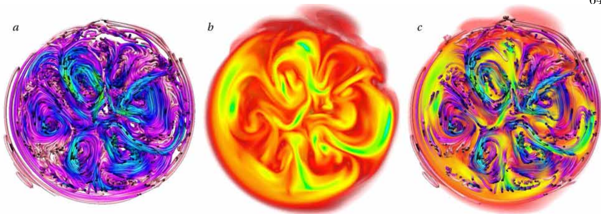
Figure 4.2: Comparing partitioning of fast flows and strong fields in a snapshot sampled in the equatorial region. ( a ) Instantaneous flow tangent lines (day 9,000). Coloring in blue/green indicates the fastest speeds ( \sim 30 \text{ m s}^{-1} ) and regions of violet/pink that of weaker flows ( \sim 5 \text{ m s}^{-1} ). Six prominent rolls are present. ( b ) Patterns of stronger magnetic energy are similar to those of the faster flows though somewhat displaced. Regions of bright green denote \sim 250 \text{ kG} fields, reddish regions \sim 30 \text{ kG} fields. ( c ) Flow lines and magnetic energy density rendered together. Regions of fast flow and strong fields exhibit notable alignment.
