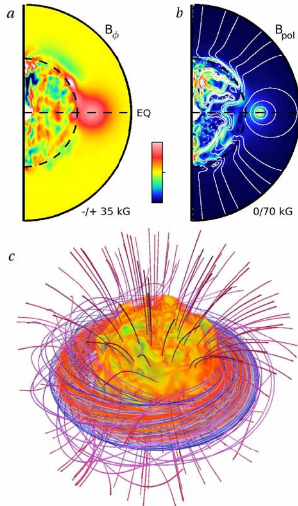
Figure 3.1: Superimposing a fossil field into the progenitor case to initiate case A. ( a ) Azimuthally-averaged B_\phi at the initial instant and ( b ) the companion poloidal field. White lines denote poloidal field lines, and the underlay the poloidal field modulus. ( c ) Magnetic energy density shown volume rendered, with the imposed field forming the outer torus of moderate field strength. Field lines correspond to those of the fossil field only.
