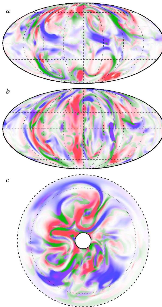
Figure 4.1: Dual rendering of kinetic energy (red) and magnetic energy (blue) near day 15,000. Regions where both quantities are strong (relative to their respective rms values) appear in green. (a) Mollweide view at the interface between the core and the radiative zone ( r=0.15R ), and (b) at mid-core, ( r=0.075R ). (c) Partial view of the equatorial plane from the pole. The dotted line denotes the edge of the convective core, and the outer dashed line r=0.19R , capturing a portion of the radiative zone (including the region of overshooting).
