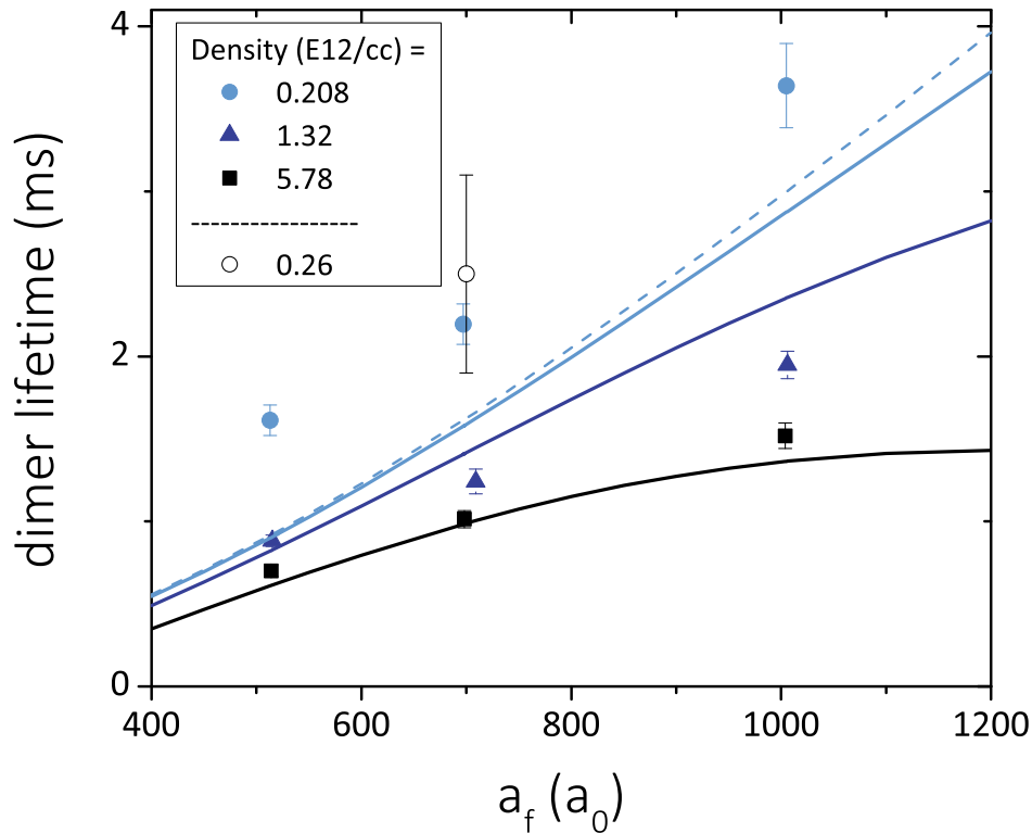
Figure 8.6: The longer of the two fitted (dimer) lifetimes as a function of a_f for initial cloud densities of n = 0.208 , 1.32 , and 5.78 \text{ E12/cc} . The solid lines represent the predicted dimer loss rates from equation 8.6, the dashed line represents the predicted dimer loss rate neglecting density-dependent atom-dimer collisions. The open circle point is a previous measurement from [93]; we see good agreement between our lowest density measurement and this previous measurement, as well as qualitative agreement between our data and the lifetime predictions, we therefore conclude that the slower of the two losses in our molecule decay data represents the Feshbach dimers in our system.
