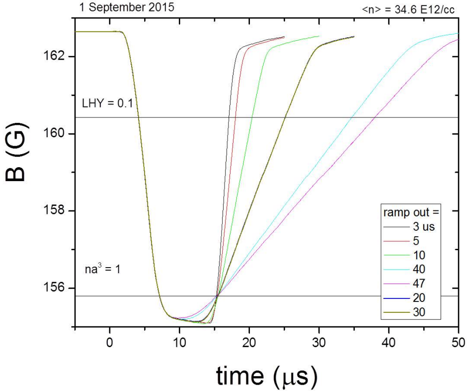
Figure 5.27: Jumps to resonance with varying r_{\text{out}} times. The dwell time was set to keep t_{\text{dwell}} the same for a density of 34.6\text{E}12/\text{cc} .
