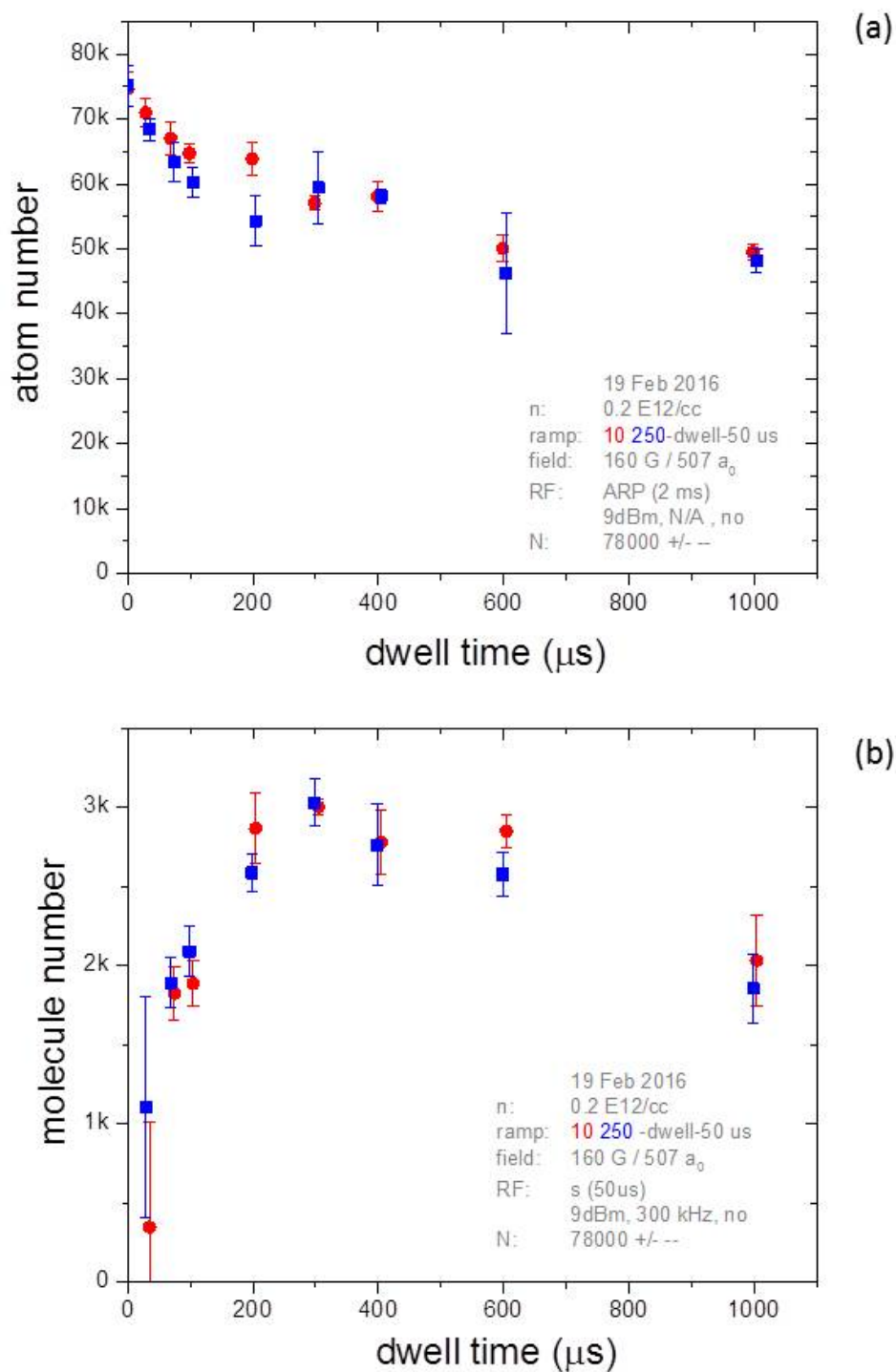
Figure 5.6: (a) The number of atoms as a function of dwell time for both a fast r_{\text{in}} (red circles) and a slow r_{\text{in}} (blue squares). We see no significant difference between the two datasets. (b) The number of molecules as a function of dwell time for both a fast r_{\text{in}} (red circles) and a slow r_{\text{in}} (blue squares). We see no significant difference between the two datasets. The density in both (a) and (b) is 0.2 E12/cc, which has a corresponding evolution time of t_n = 510 \mu\text{s} .
