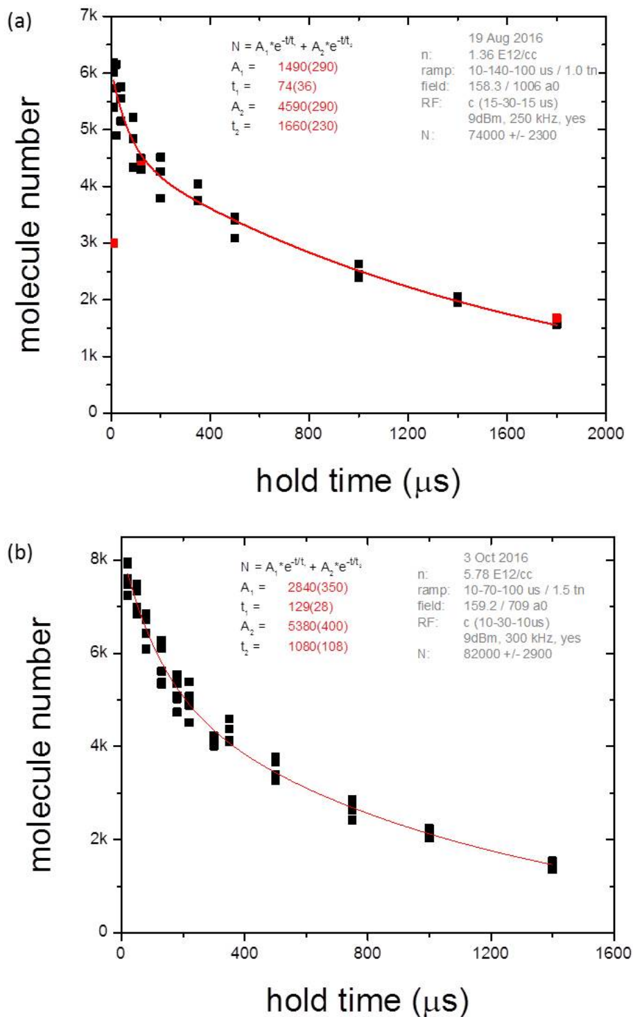
Figure 8.2: (a) The molecular loss from a n = 1.32 E12/cc cloud ramped out to a_f \approx 1000 a_0 . Comparing the summed two exponential fit with that in figure 8.1 for the same same n , we see that the fast loss remains unchanged within error while the slower loss becomes even slower. (b) The molecular loss from a n = 5.75 E12/cc cloud ramped out to a_f \approx 700 a_0 . Comparing this to the other a_f = 700 a_0 datasets of different densities in the previous figure, the fast loss remains unchanged within error while the slow loss has a shorter lifetime at this higher density.
