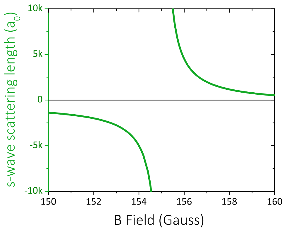
Figure 2.1: The two-body s-wave scattering length near the 155 G Feshbach resonance of ^{85}\text{Rb} .
