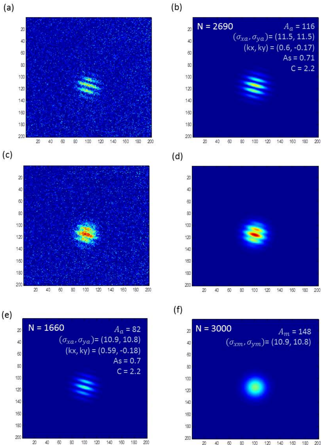
Figure 6.10: (a) The stripes across an atom (no molecules) cloud at 700 a_0 after a 9 dBm, 50 \mu\text{s} microwave pulse detuning 300 kHz from resonance. (b) A fit to the atom cloud shows that 2690 atoms were transferred to the imaging state. (c) Atom stripes appear across a cloud of both atoms and molecules, created by a 510 \mu\text{s} dwell time ( \sim 1 t_n for n = 0.2 \text{ E12/cc} cloud) on resonance and a ramp time = 100 \mu\text{s} to 700 a_0 . (d) A fit to the molecule + atom cloud. (e) The atom contribution to the atom+molecule fit predicts 1660 atoms. After accounting for loss at unitarity we expect 65% of the original atom number. (f) The molecule contribution is about 3000 molecules.
