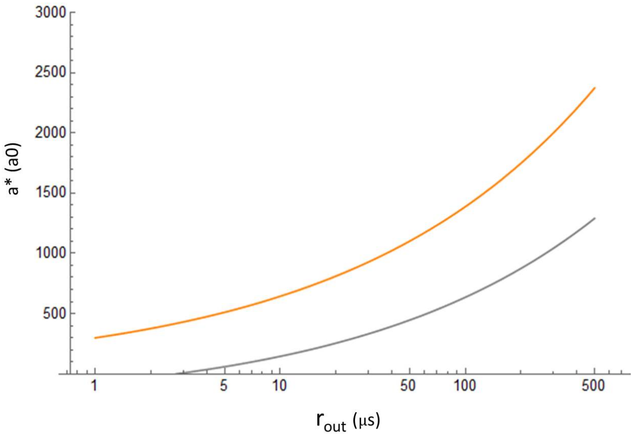
Figure 7.8: The calculated a_* as a function of r_{\text{out}} for constant \Delta_B , assuming a linear a(B) approximation (orange) given by equation (7.1), or a more accurate a(B) relation (gray) given by equation (7.5). The latter has lower values of a_* , meaning that more of the total ramp time is adiabatic, and therefore predicts that less atoms will be swept into the shallow molecule state.
