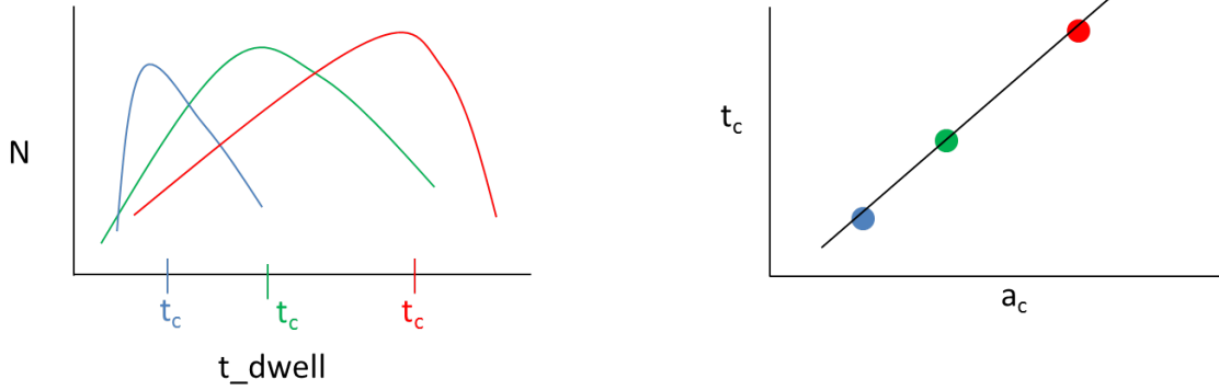
Figure 9.14: (a) Qualitative prediction of the number of molecules produced as a function of t_{\text{dwell}} for ramp outs with various values of a_c (corresponding the a_c lines drawn in figure 9.13). The number will be maximum when a' = a_c . We define the dwell time that yields maximum number as t_c . (b) Now plotting t_c as a function of a_c should yield a linear line if the growth rate on resonance is linear. The inverse of this function yields a' as a function of t_{\text{dwell}} . We could know how the molecular size changes as the cloud evolves at unitarity.
