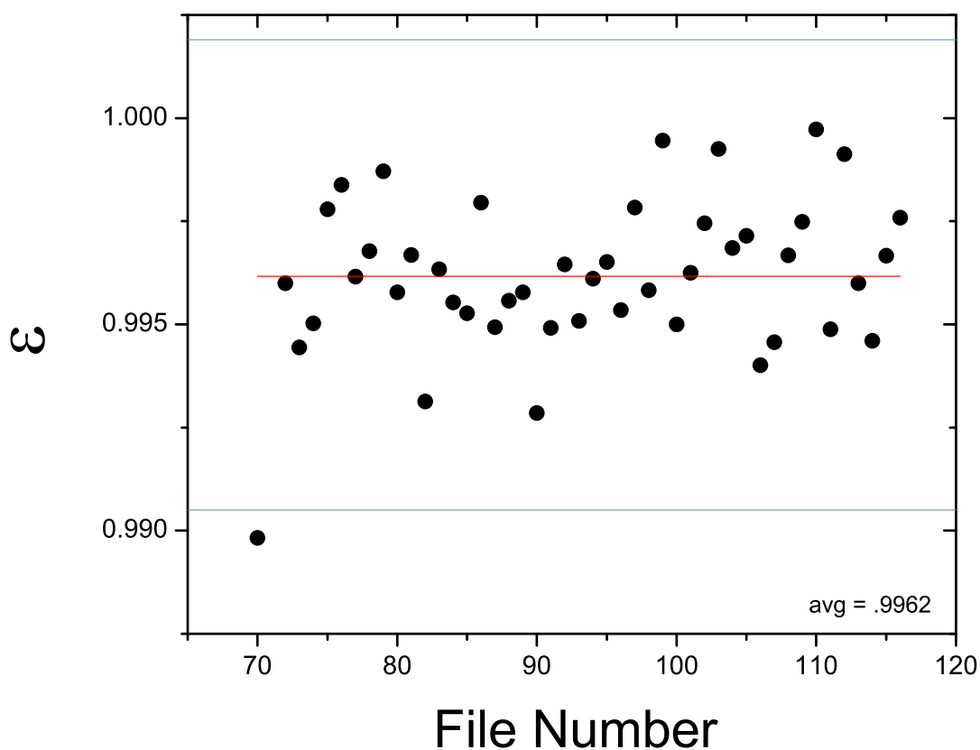
Figure 3.14: The average value of \epsilon , evaluated with a 75 pixel box; the lines represent \pm 3 \sigma . The average value of \epsilon is about 0.996, meaning that 99.6% of the incident light in the light frame is also present in the shadow frame.
