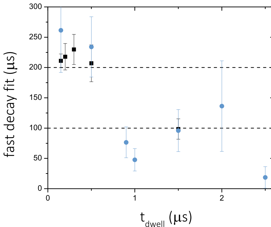
Figure 9.9: The fitted trimer lifetime measured in n = 1.32 \text{ E12/cc} ( t_n = 146 \mu\text{s} ) clouds at a_f = 700 a_0 for various resonance dwell times. For these fits, we fixed t_2 to 1250 \mu\text{s} . The black squares are fits from the high-density-of points data, like those from figure 9.5; the blue circles are the fits from less full datasets from Appendix C and therefore have larger error bars. We see that the trimer lifetime fits near the expected value of 100 \mu\text{s} when t_{\text{dwell}} \geq 1 t_n , and fits near 200 \mu\text{s} from all shorter t_{\text{dwell}} 's. It is particularly interesting that this lifetime doubles as quick as a step function, rather than slowly changing.
