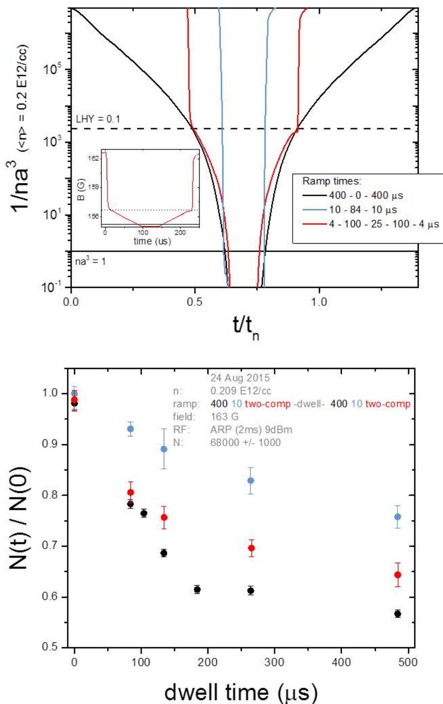
Figure 5.30: (a) There are three ramps in this experiment: two were single-component ramps characterized as 10 \mu s “fast ramp” (blue) and a 400 \mu s “slow ramp” (black) and the third ramp was a two-component ramp (red) that matched the “slow” ramp for na^3 \geq 0.000431 and the fast ramp for na^3 < 0.000431 . The inset shows this two-component ramp on a linear scale. (b) The number of atoms that returned as a function of dwell time for each respective ramp.
