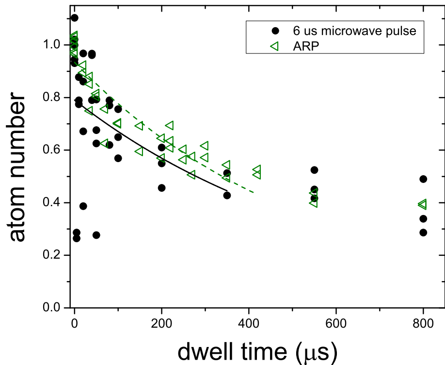
Figure 5.9: The number of atoms transferred to the imaging state via a 6 \mu\text{s} square microwave pulse on resonance (black circles) or a 2 ms ARP after a 5 \mu\text{s} ramp back to weak interactions (open green triangles) as a function of dwell time. We trust that the ARP transfers all of the surviving atoms to the imaging state, yet the ramp back to weak interactions may itself lose atoms. The ARP number is therefore a minimum number expectation. Because the on-resonance 6 \mu\text{s} microwave pulse transfers less atoms at short dwell times, we conclude that this imaging method is compromised by field noise.
