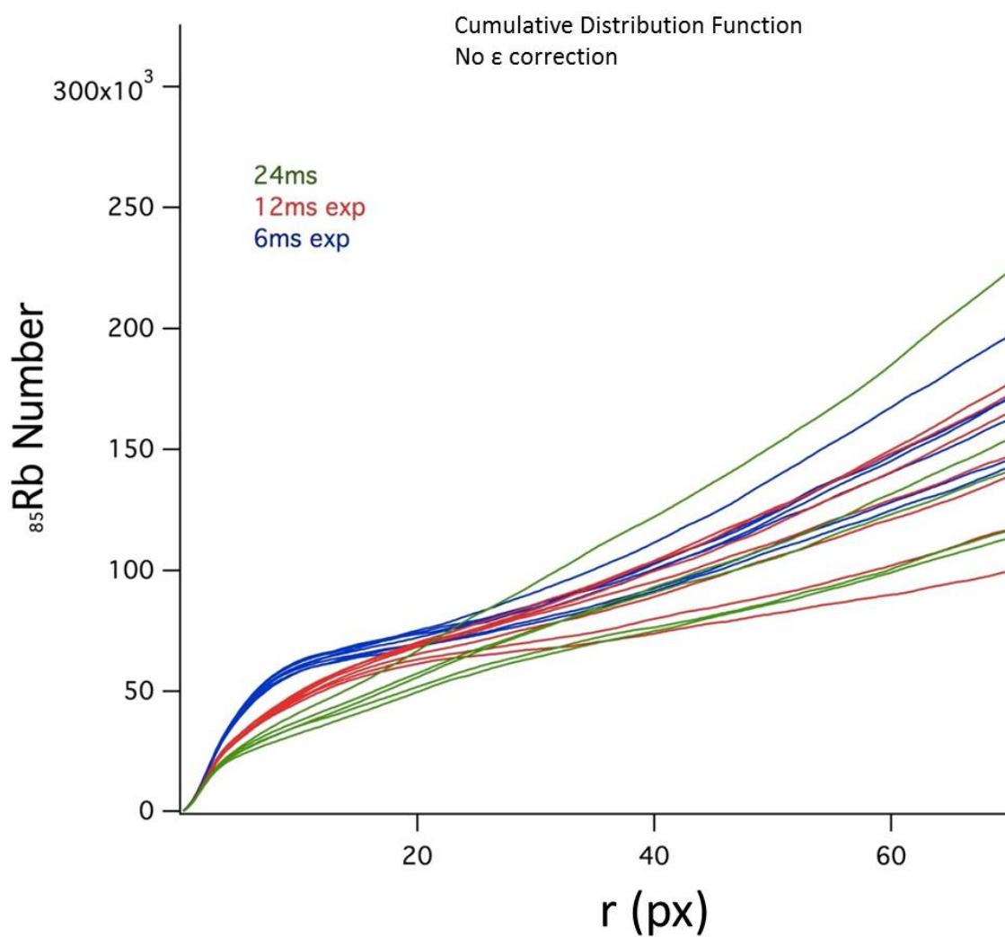
Figure 3.17: The cumulative distribution functions (CDFs) of many condensates after a 5-100-5 \mu\text{s} resonance jump. The clouds were expanded in TOF for 6 (blue), 12 (red) or 24 (green) ms. With no \epsilon correction, we see that the CDFs continue to increase at large radii, indicating that the optical density images have a positive background.
