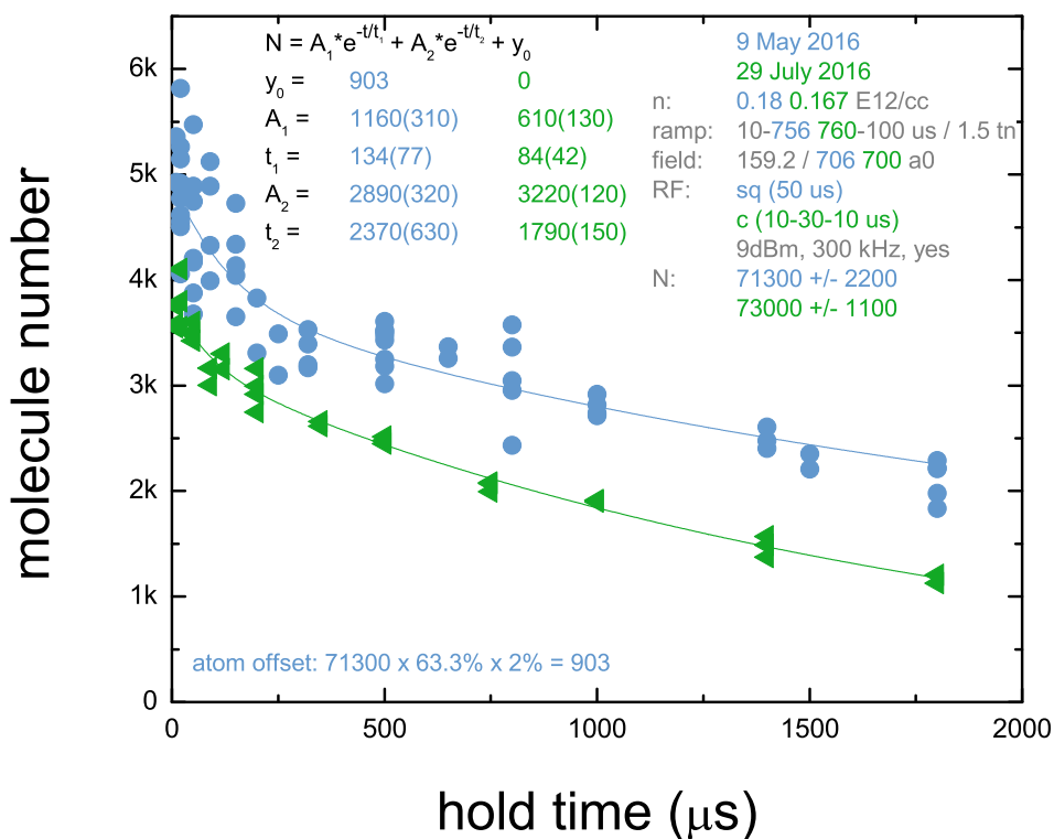
Figure 6.21: The number of molecules (and atoms) imaged after a (10-30-10 \mu s ) curved RF pulse (green triangle) or a 50 \mu s square RF pulse (blue point) after a t_{\text{dwell}} = 1.5 t_n evolution on resonance and ramp time = 100 \mu s to 700 a_0 . Both datasets account for the falling cloud with frequency tracking. In addition to the molecules, there are about 900 atoms transferred to the imaging state for the square dataset.
