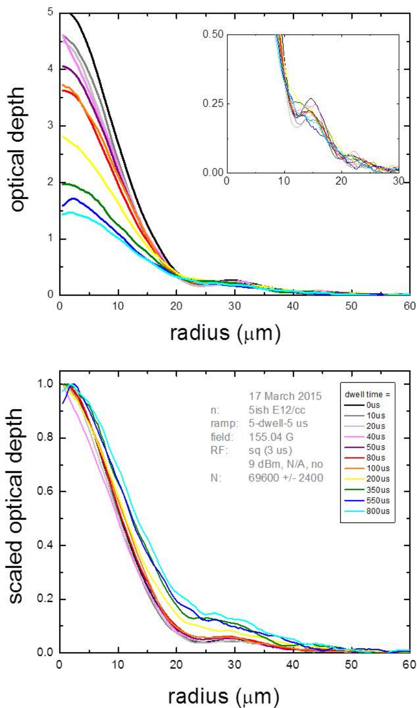
Figure 5.15: (a) The azimuthal averages for the standard density expansion data. The data were azimuthally averaged before clouds with common dwell times were averaged together. The most striking characteristic that evolves with dwell time is the drop in peak optical density. The inset zooms in on the bump that occurs in all datasets around 15 pixels ( \text{px} = 1.996 \mu\text{m} ) (b) The azimuthal averages scaled by their peak optical depth. This scaling emphasizes how the tail at large radii grows over time, causing the cloud to deviate from a typical Gaussian shape .
