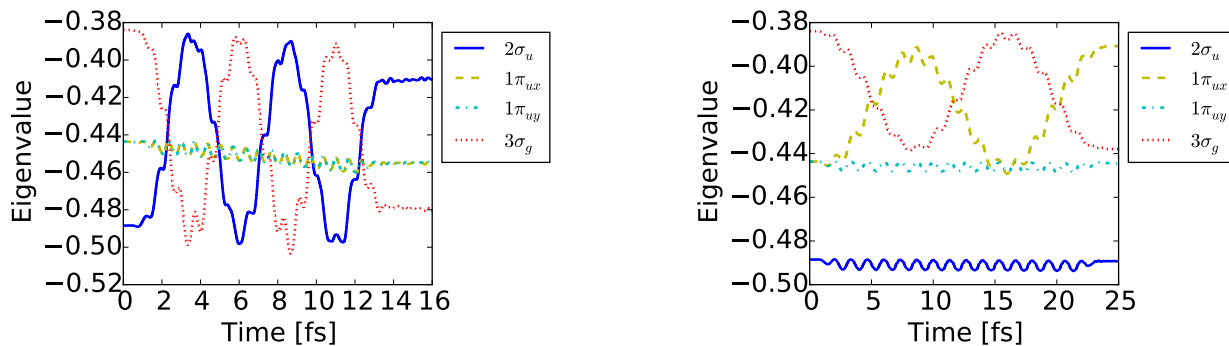
Figure 4.9: Instantaneous eigenvalues of Kohn-Sham Hamiltonian for N_2 valence orbitals for 400 nm laser field at parallel orientation (left) with intensity of 5 \times 10^{13} \text{ W/cm}^2 and 800 at perpendicular orientation (right) with intensity of 5 \times 10^{13} \text{ W/cm}^2 . Only the relevant KS orbitals, which exhibit significant response to the laser field, are shown with their labels.
