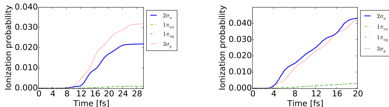
Figure 4.5: Comparison of ionization from N_2 between \sin^2 (left) and trapezoidal (right) envelope. Wavelength is 400 nm and intensity is 8 \times 10^{13} W/cm 2 with polarization parallel to the molecular axis of N_2 . Only the relevant KS orbitals which possess an important response to the laser field are shown with their labels.
