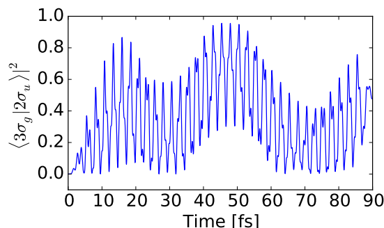
Figure 5.6: The projection from HOMO-2 to HOMO of \text{N}_2^+ for two-color laser field: 400 nm laser field at I = 1 \times 10^{12} \text{ W/cm}^2 and 800 nm laser field at I = 1 \times 10^{14} \text{ W/cm}^2 .
