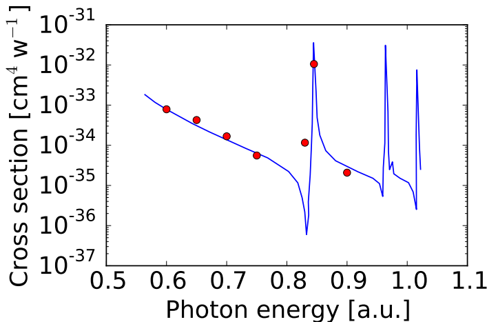
Figure 6.7: Cross section of two-photon ionization from H_2^+ at laser intensity I=1.76 \times 10^{13} W/cm 2 . The solid curve is adapted from [211, 244] and the red dot is our calculations.
