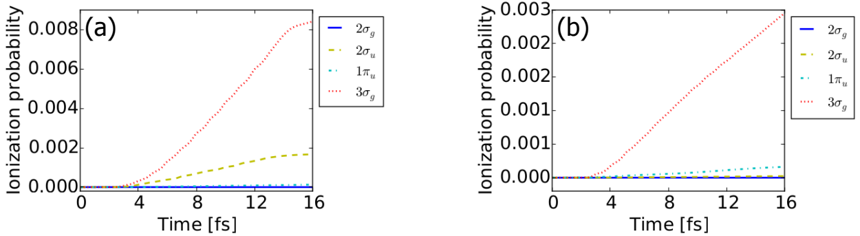
Figure 4.1: Ionization from KS orbitals of \text{N}_2 for parallel (a) and perpendicular (b) alignment with respect to external laser field polarization. The laser field parameters: wavelength of 600 nm and intensity of 5 \times 10^{13} \text{ W/cm}^2 .
