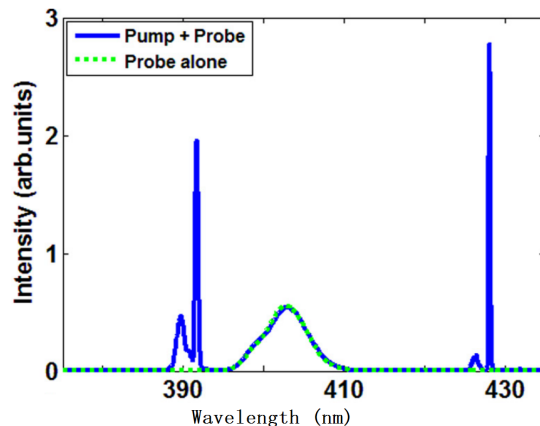
Figure 4.13: The spectra captured with (blue) and without (green) the pump pulse. Laser parameters Adapted from [186].
