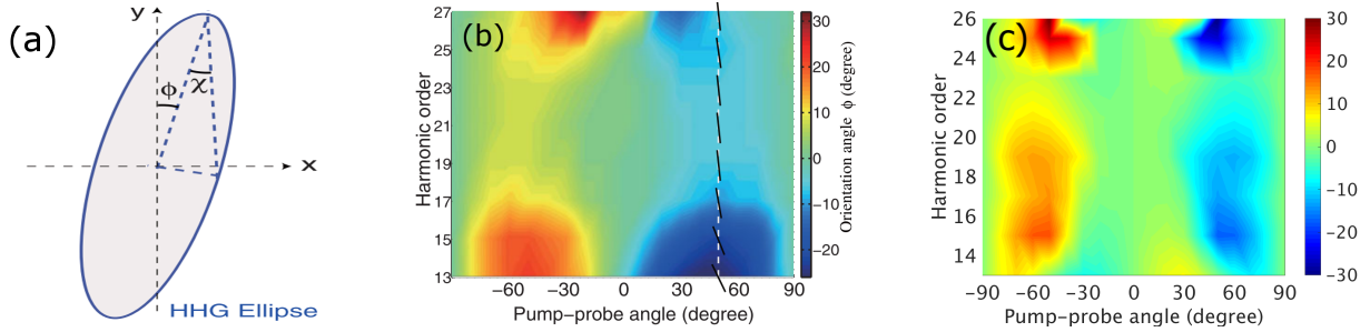
Figure 3.34: Illustration of high harmonic ellipticity orientation angle (a), experimental results of ellipticity orientation angle from \text{CO}_2 (b), adapted from [165], and our simulation results (c).
