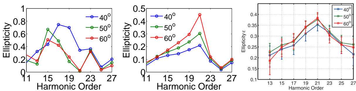
Figure 3.27: Ellipticity of high-order harmonics as a function of the harmonic orders for three molecular alignment angles at \lambda = 800 \text{ nm} and peak intensity of I_o = 1 \times 10^{14} \text{ W/cm}^2 . Comparison of results in which no average (left panel) and a proper average (middle panel) over the distribution of the alignment in the molecular ensemble has been taken into account and experimental results (at 2 \times 10^{14} \text{ W/cm}^2 )(right), adapted from [165].
