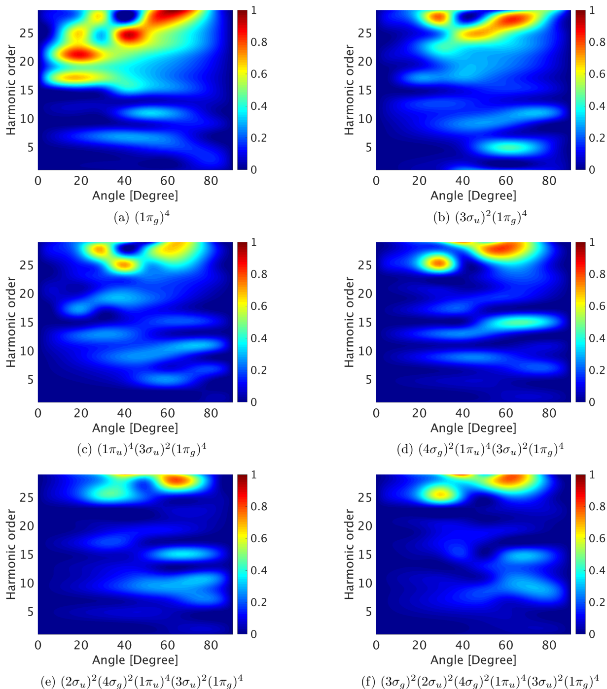
Figure 3.36: Ellipticity of harmonics as a function of alignment angle for \text{CO}_2 . Starting with the results from HOMO only (upper left), contributions from inner valence orbitals are added step by step in the other panels (as indicated). A proper average over the distribution of the alignment in the molecular ensemble is made. Applied laser field is at wavelength of 800 nm and intensity of 1.5 \times 10^{14} \text{ W/cm}^2 with 30 fs pulse length.
