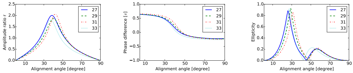
Figure 3.24: The amplitude ratio r (left), phase difference \delta (middle), and the ellipticity (right) of high-order harmonics from \text{H}_2^+ in a laser field at wavelength of 800 nm and intensity 3 \times 10^{14} \text{ W/cm}^2 .
