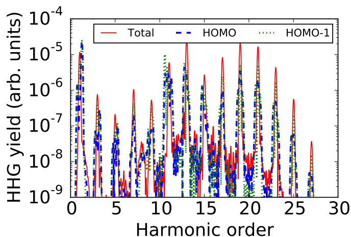
Figure 3.3: The high harmonic spectra of \text{N}_2 from its two outermost states HOMO ( 3\sigma_g ) (blue dash) and HOMO-1 ( 1\pi_u ) (green dots). The total spectra from these two orbitals are also plotted (red solid line). The wavelength of the laser field is 800 nm at intensity of 2 \times 10^{14} \text{ W/cm}^2 with polarization perpendicular to the molecular axis.
