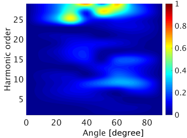
Figure 3.35: Ellipticity of high harmonics as function of alignment angle for \text{CO}_2 for a laser field at \lambda = 800 \text{ nm} and I = 1.5 \times 10^{14} \text{ W/cm}^2 .
