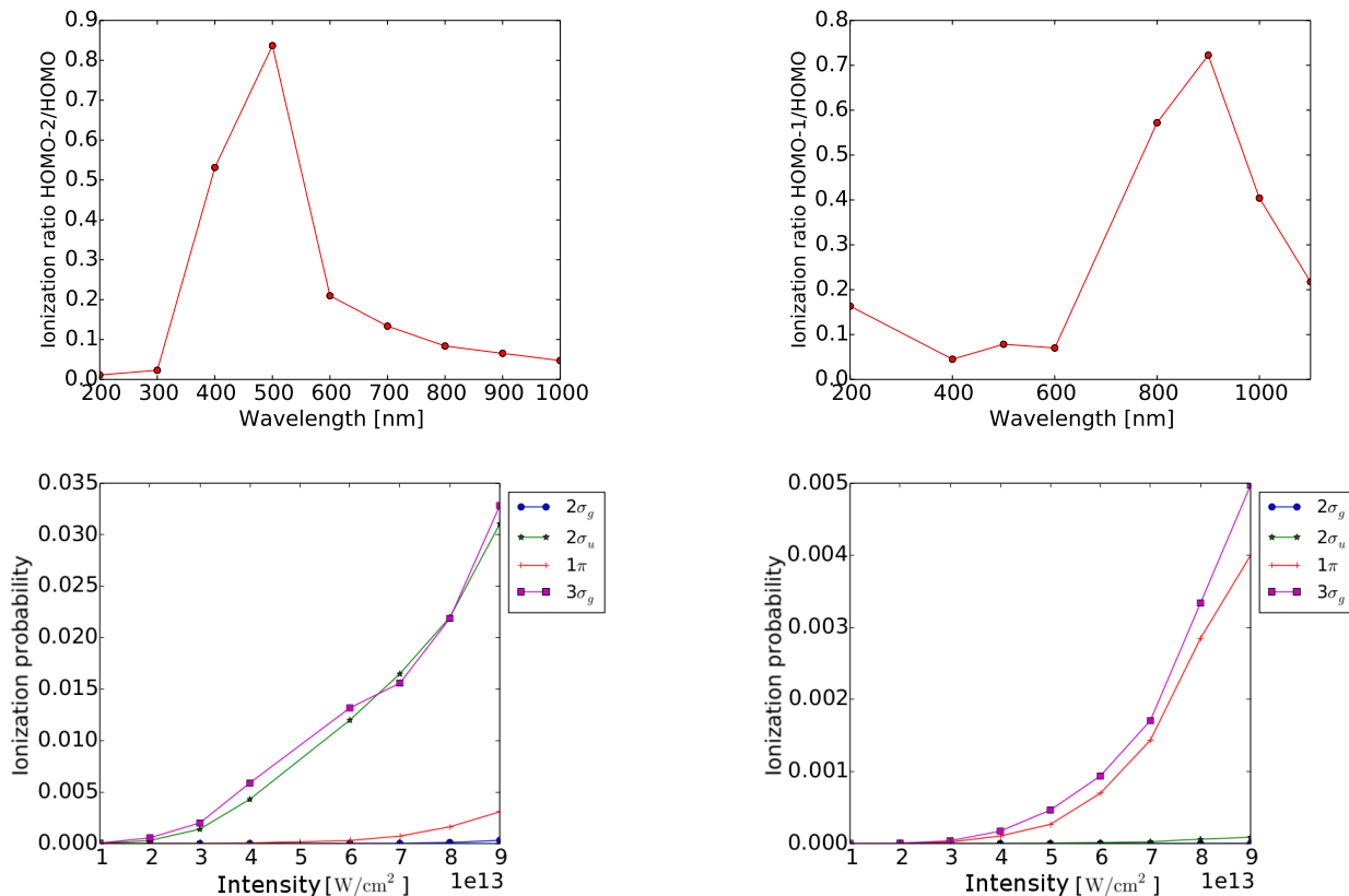
Figure 4.8: Upper panels: Ratio of ionization yields between HOMO-2 and HOMO (left) and HOMO-1 and HOMO (right) of N_2 as a function of laser wavelength at intensity of 5 \times 10^{13} \text{ W/cm}^2 and a pulse length of 14 fs. Lower panels: Ionization yields for HOMO and inner valence orbitals as a function of intensity at wavelength of 400 nm (left) and 800 nm (right). Panels on left are for parallel alignment, while panels on right are for perpendicular alignment.
