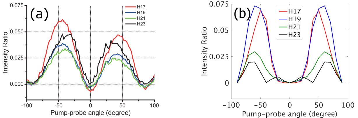
Figure 3.33: Intensity ratio of perpendicular to parallel component. Comparison between experimental result (a) adapted from [165], and our simulation result (b).
