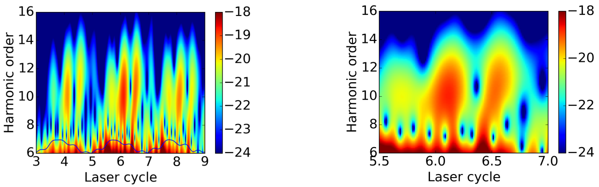
Figure 3.16: Wavelet analysis of high harmonic generation in N_2^+ aligned parallel to the polarization direction of the laser field. Laser parameters are the same as in Fig. 3.6.
