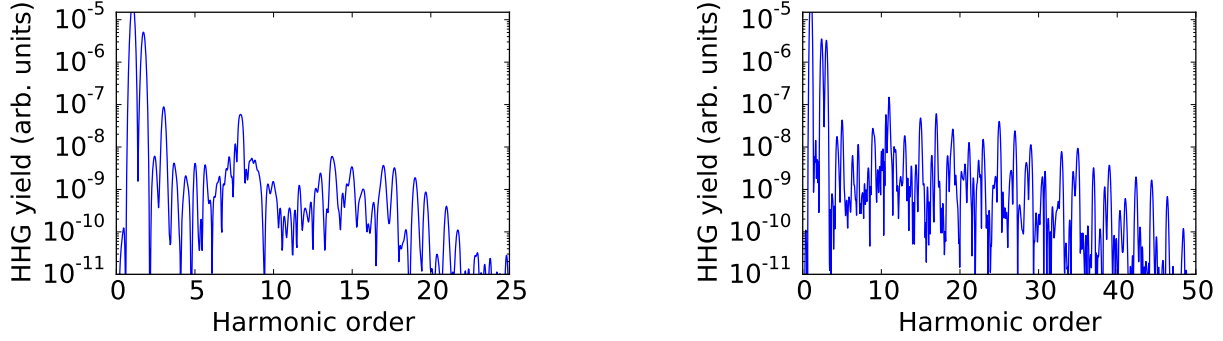
Figure 3.9: HHG spectra from \text{N}_2^+ for laser field at wavelength of 600 nm (left) with intensity of 1 \times 10^{14} \text{ W/cm}^2 and at wavelength of 800 nm (right) with intensity of 2 \times 10^{14} \text{ W/cm}^2 . Molecular axis is oriented parallel to the polarization of laser field. Pulse length is 20 fs.
