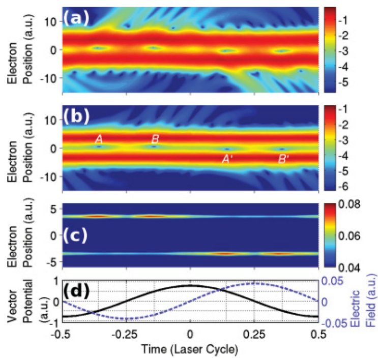
Figure 5.2: Multiburst ionization from \text{H}_2^+ at internuclear distance of R=7.0 a.u. along the molecular axis in a strong laser field (shown in d) using (a) 1D model and (b, c) 2D model. Adapted from [203]
