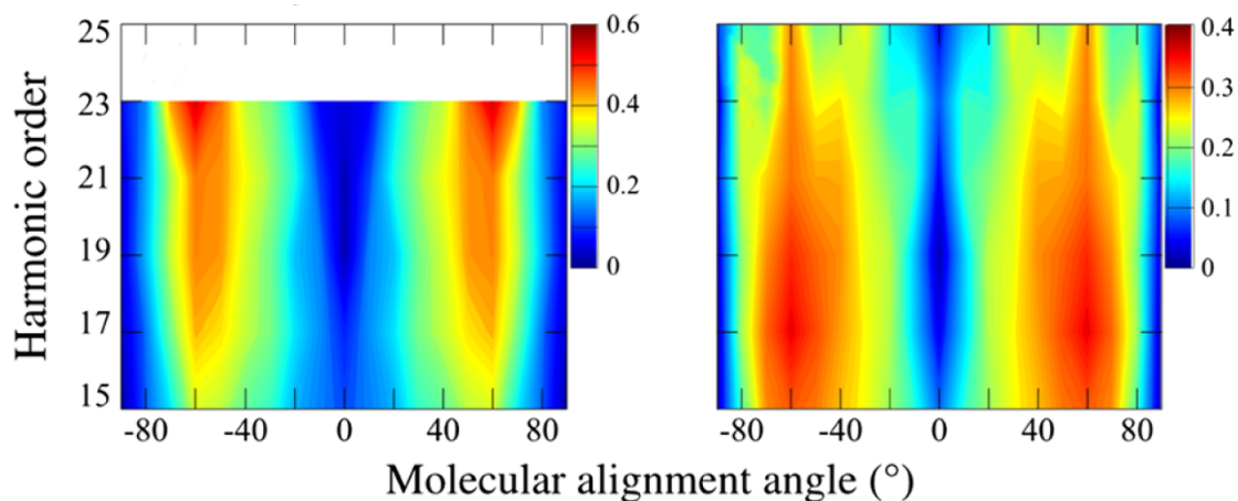
Figure 3.28: Ellipticity from N_2 with 800 nm laser field at intensity of 8 \times 10^{13} \text{ W/cm}^2 (left) and 1 \times 10^{14} \text{ W/cm}^2 (right), adapted from [154].
