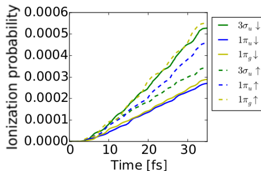
(b) \text{CO}_2^+ with |1\pi_g \uparrow\rangle partially occupied. Laser parameters: \lambda=350 nm, I = 1 \times 10^{14} W/cm 2 . |1\pi_u \uparrow\rangle and |1\pi_g \uparrow\rangle are coupled. For the \pi_g and \pi_u orbital, ionization is normalized by initial number of electrons.
