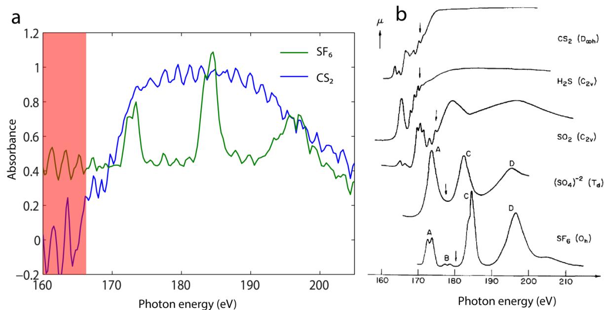
Figure 5.9 (a) NEXAFS of CS 2 and SF 6 obtained from our HHG Soft X-ray. (b) Synchrotron data for CS 2 , H 2 S, SO 2 , (SO 4 ) 2- , and SF 6 NEXAFS, adapted from [126].
